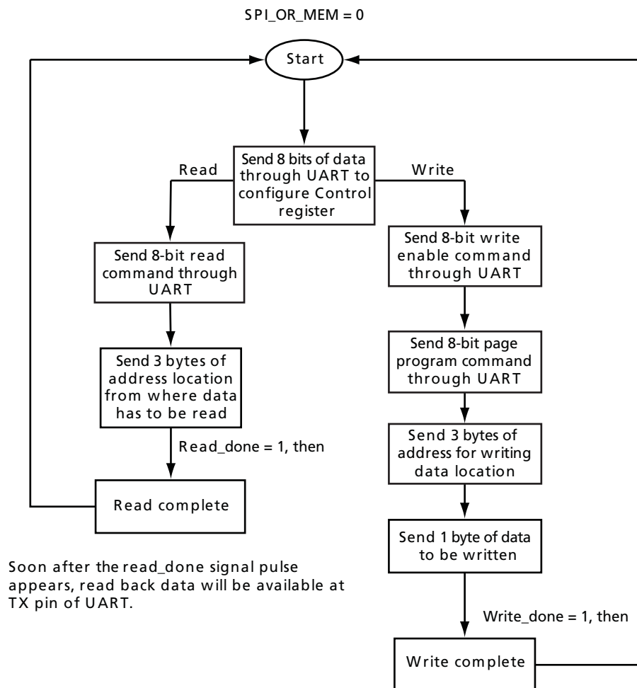
Figure 3 • SPI Read and Write Cycle Mode 0
