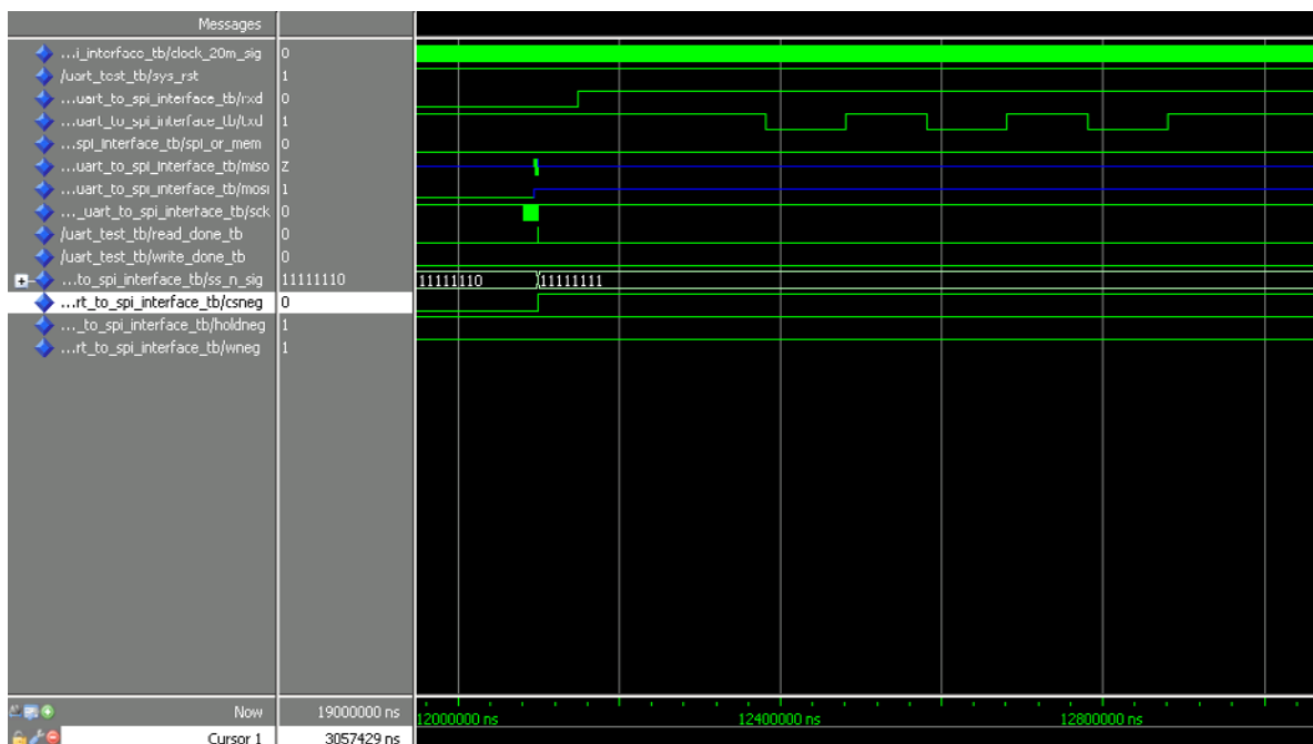
Figure 6 • Read Cycle
