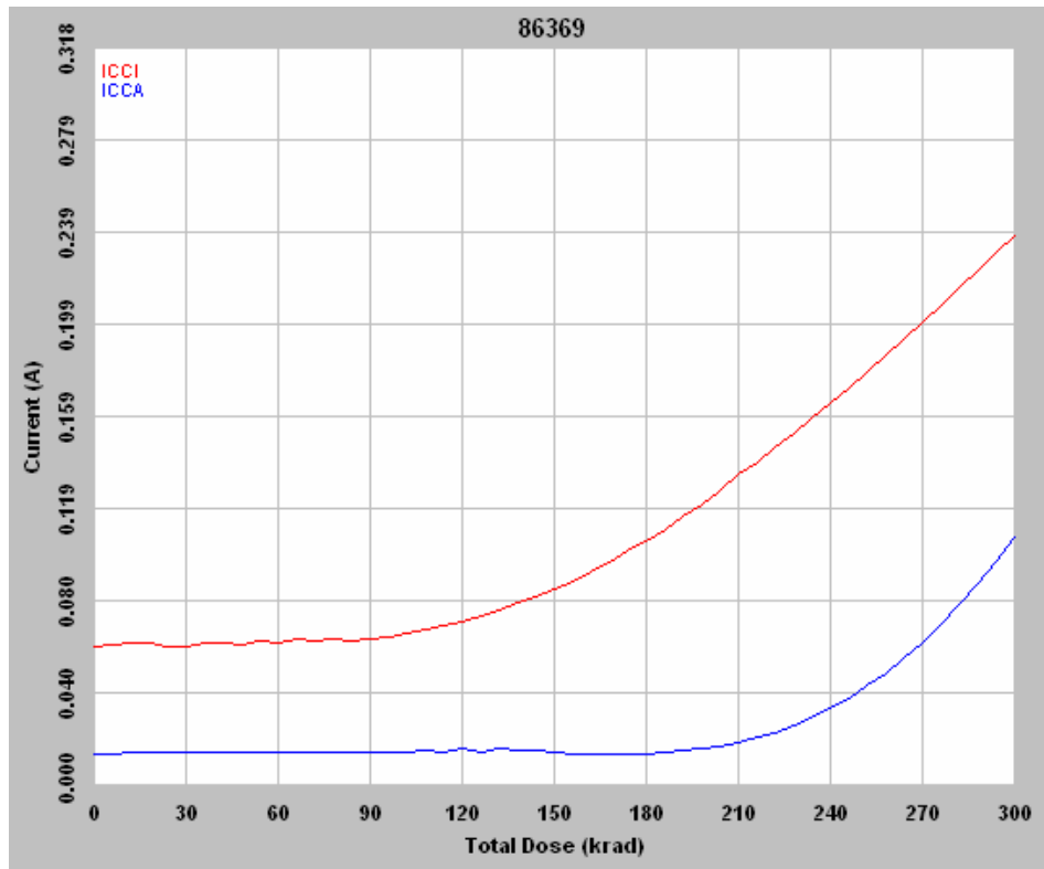
Figure 6 DUT 86369 in-flux I_{CCA} and I_{CCI}
