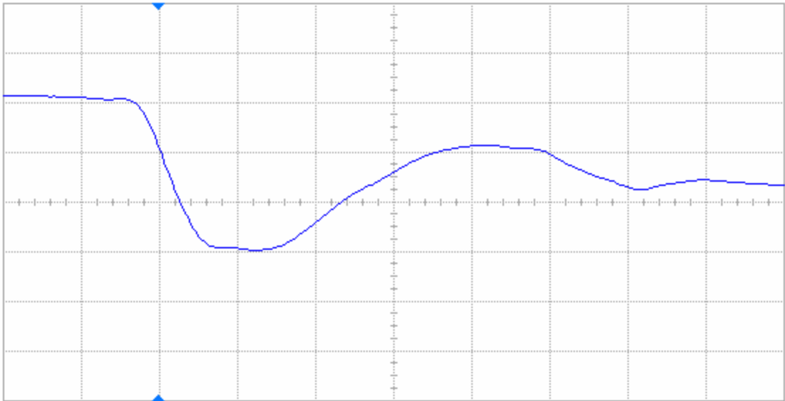
Figure 14(b) DUT 86299 post-annealing falling edge, abscissa scale is 2 V/div and ordinate scale is 2 ns/div.
