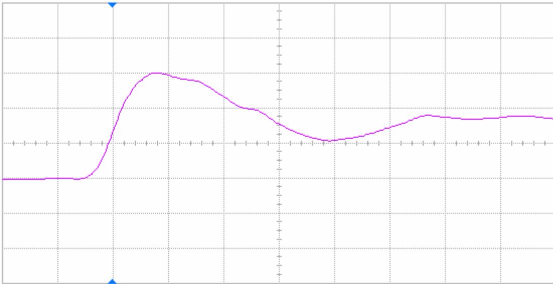
Figure 7(a) DUT 86277 pre-irradiation rising edge, abscissa scale is 2 V/div and ordinate scale is 2 ns/div.
