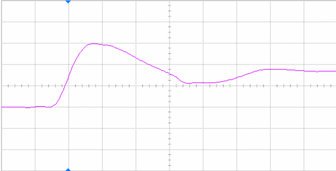
Figure 8(a) DUT 86299 pre-irradiation rising edge, abscissa scale is 2 V/div and ordinate scale is 2 ns/div.
