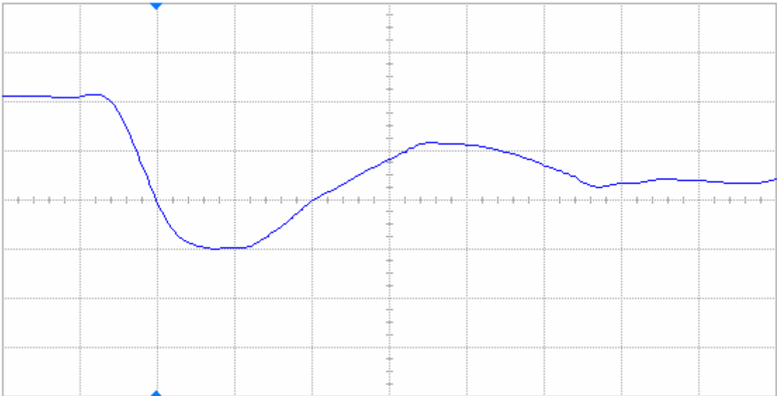
Figure 15(b) DUT 86321 post-annealing falling edge, abscissa scale is 2 V/div and ordinate scale is 2 ns/div.
