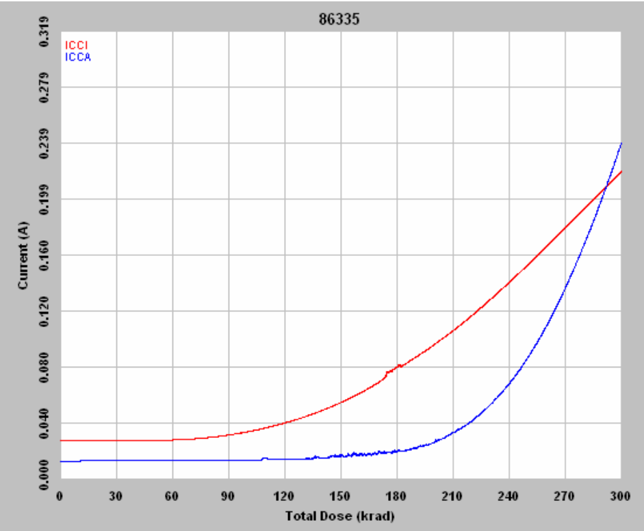
Figure 5 DUT 86335 in-flux I_{CCA} and I_{CCI}
