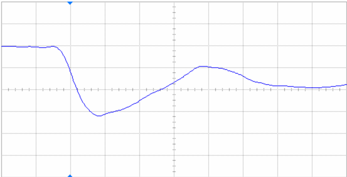
Figure 16(b) DUT 86331 post-annealing falling edge, abscissa scale is 2 V/div and ordinate scale is 2 ns/div.
