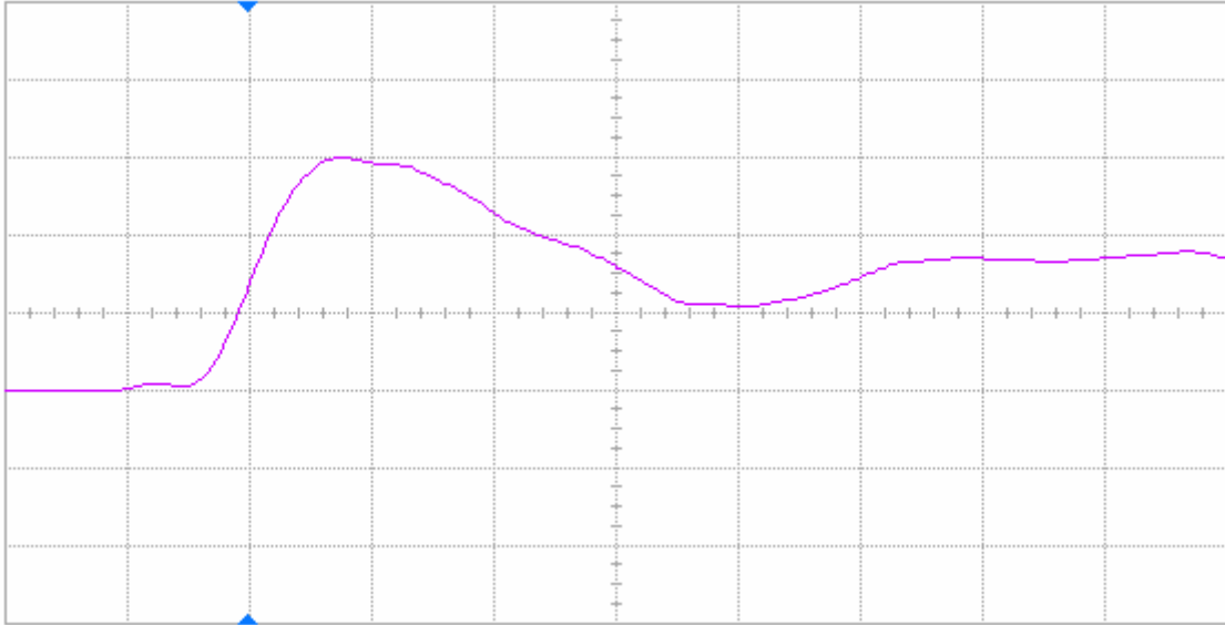
Figure 10(a) DUT 86331 pre-irradiation rising edge, abscissa scale is 2 V/div and ordinate scale is 2 ns/div.
