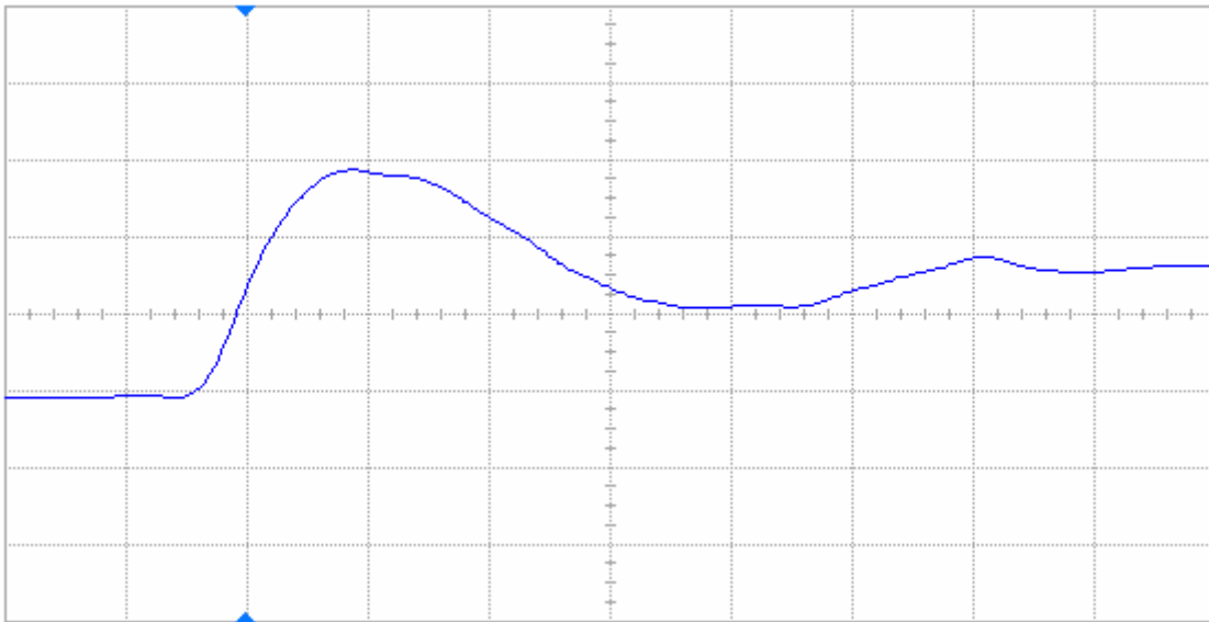
Figure 7(b) DUT 86277 post-annealing rising edge, abscissa scale is 2 V/div and ordinate scale is 2 ns/div.
