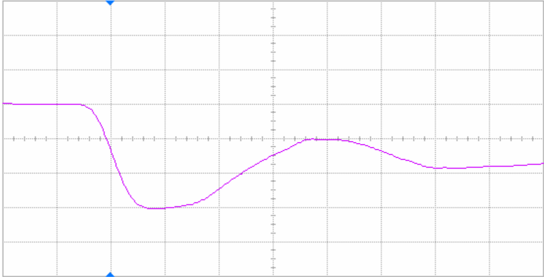
Figure 15(a) DUT 86321 pre-irradiation falling edge, abscissa scale is 2 V/div and ordinate scale is 2 ns/div.
