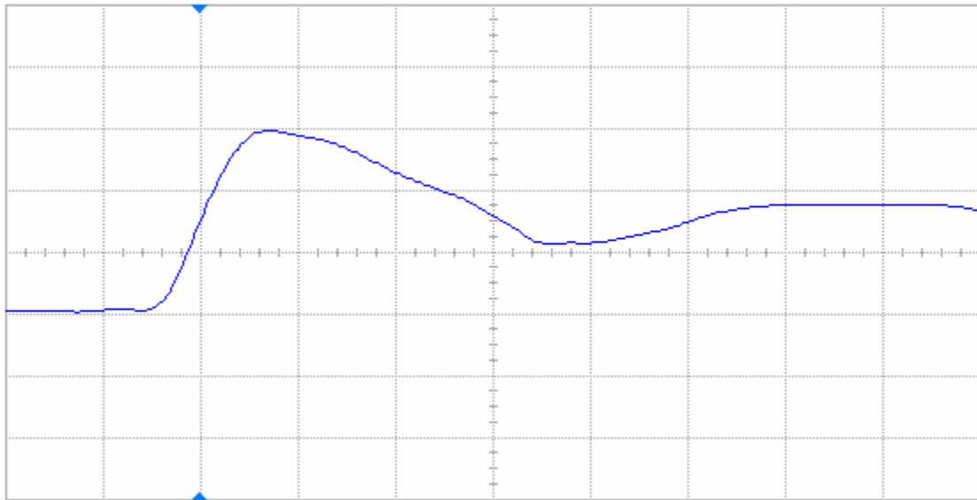
Figure 11(b) DUT 86335 post-annealing rising edge, abscissa scale is 2 V/div and ordinate scale is 2 ns/div.
