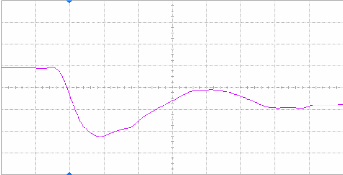
Figure 14(a) DUT 86299 pre-irradiation falling edge, abscissa scale is 2 V/div and ordinate scale is 2 ns/div.
