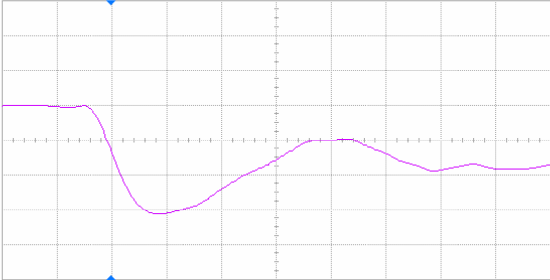
Figure 18(a) DUT 86369 pre-irradiation falling edge, abscissa scale is 2 V/div and ordinate scale is 2 ns/div.
