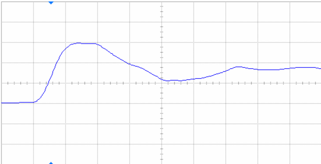
Figure 8(b) DUT 86299 post-annealing rising edge, abscissa scale is 2 V/div and ordinate scale is 2 ns/div.
