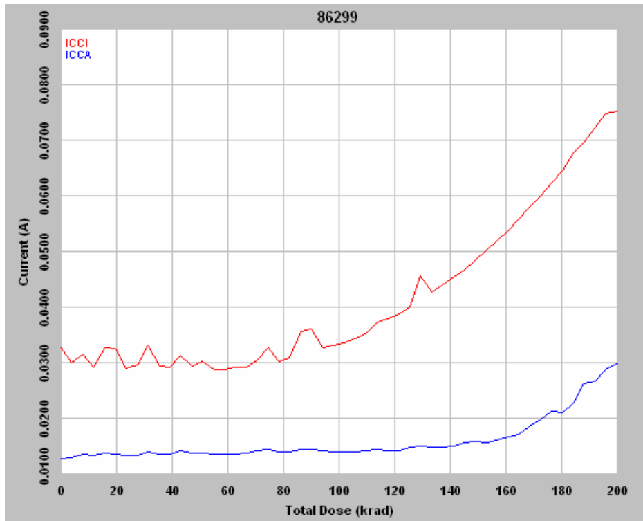
Figure 2 DUT 86299 in-flux I_{CCA} and I_{CCI}
