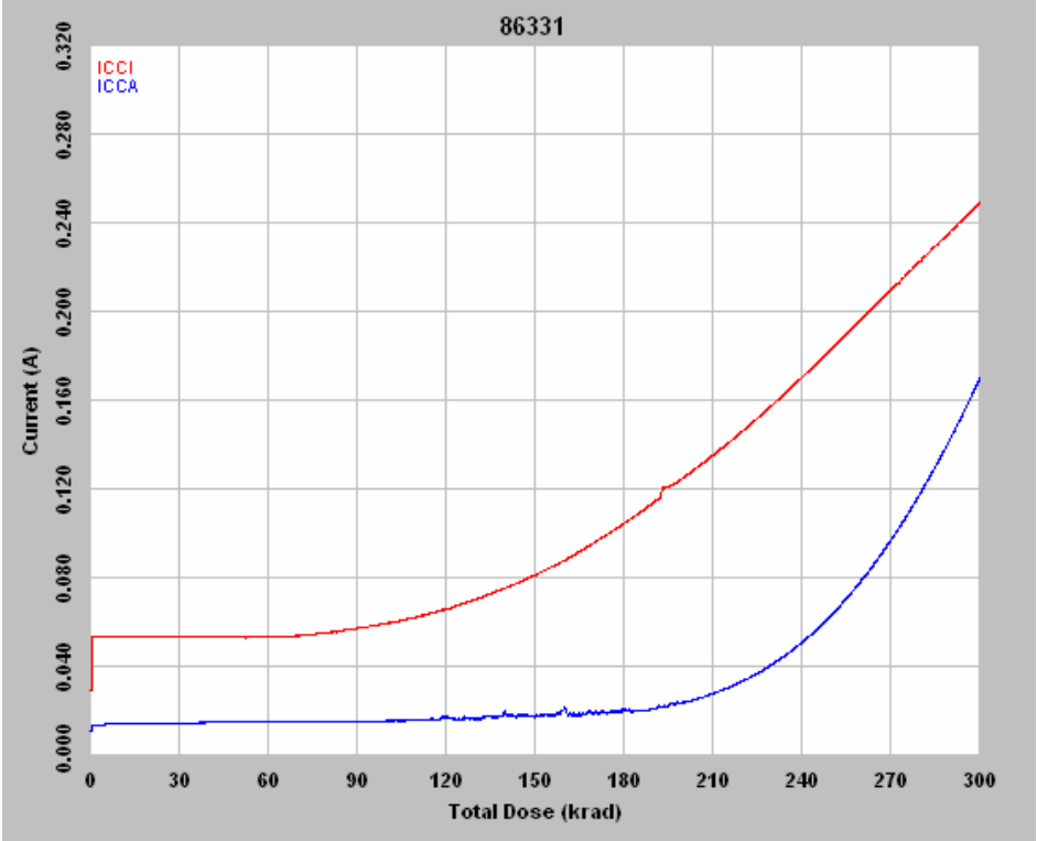
Figure 4 DUT 86331 in-flux I_{CCA} and I_{CCI}
