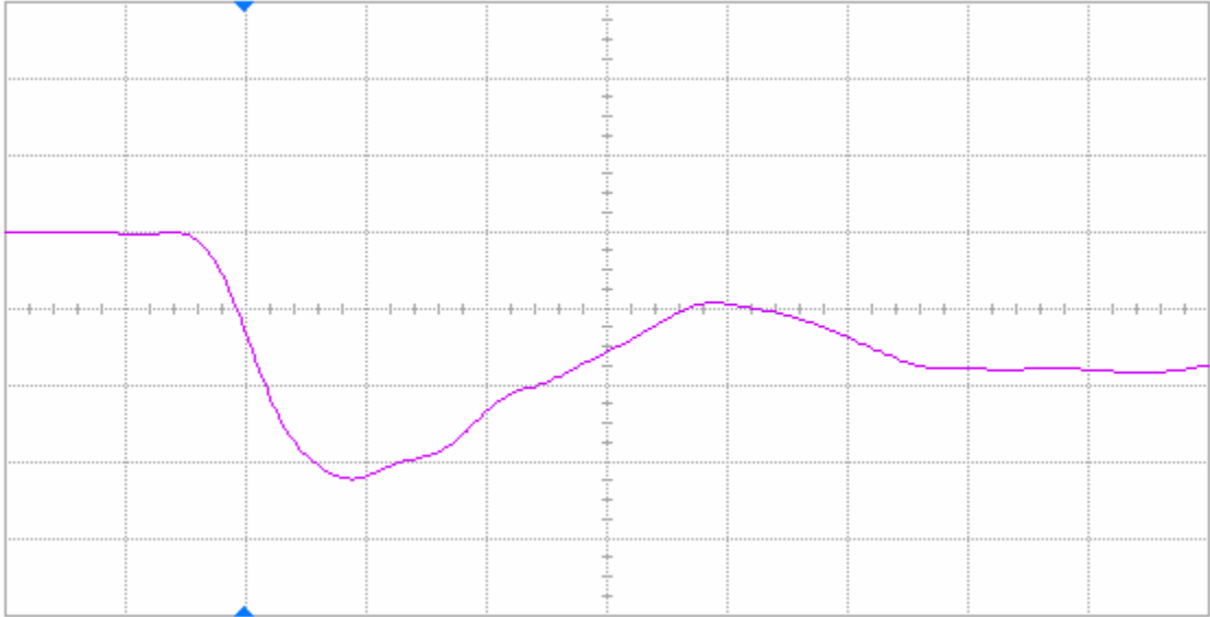
Figure 17(a) DUT 86335 pre-irradiation falling edge, abscissa scale is 2 V/div and ordinate scale is 2 ns/div.
