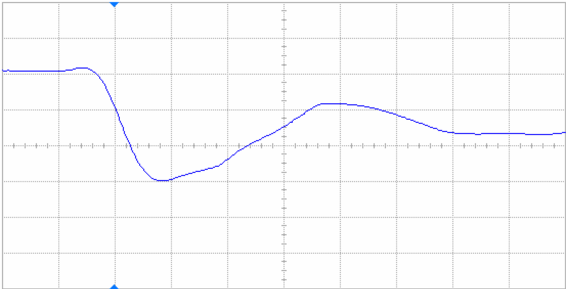
Figure 17(b) DUT 86335 post-annealing falling edge, abscissa scale is 2 V/div and ordinate scale is 2 ns/div.
