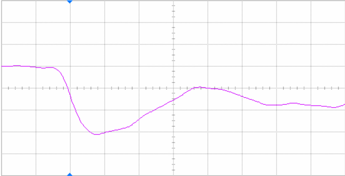
Figure 16(a) DUT 86331 pre-irradiation falling edge, abscissa scale is 2 V/div and ordinate scale is 2 ns/div.
