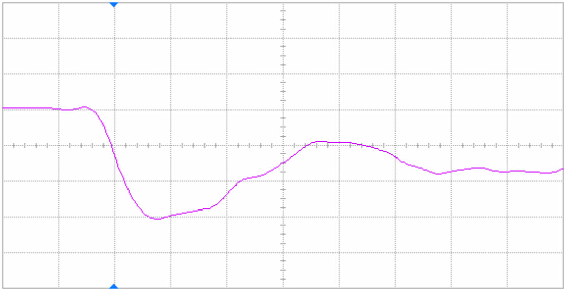
Figure 13(a) DUT 86277 pre-irradiation falling edge, abscissa scale is 2 V/div and ordinate scale is 2 ns/div.
