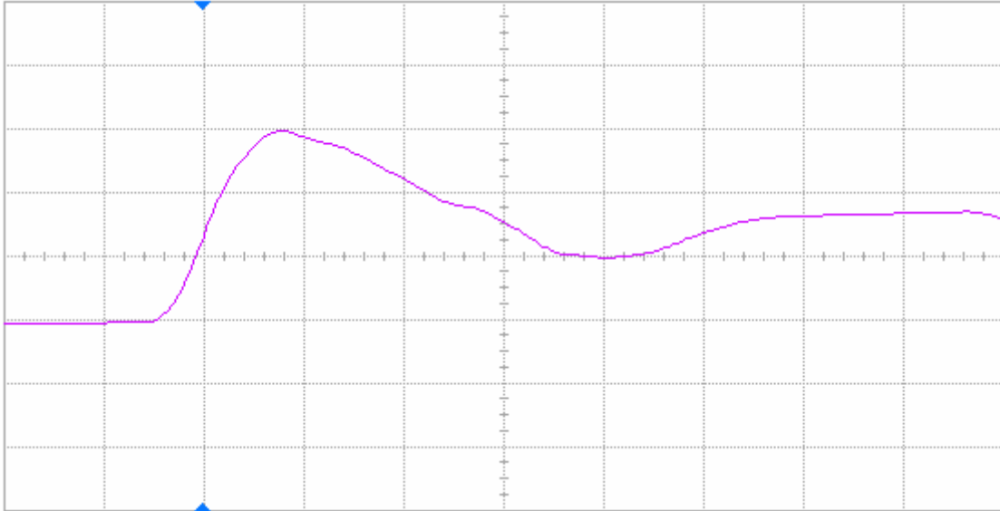
Figure 11(a) DUT 86335 pre-irradiation rising edge, abscissa scale is 2 V/div and ordinate scale is 2 ns/div.
