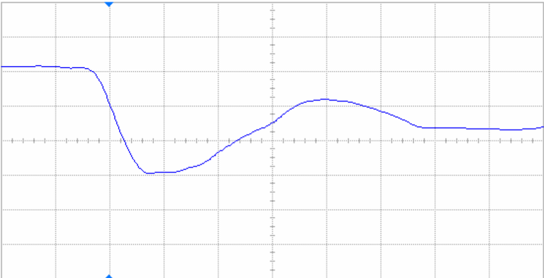
Figure 18(b) DUT 86369 post-annealing falling edge, abscissa scale is 2 V/div and ordinate scale is 2 ns/div.
