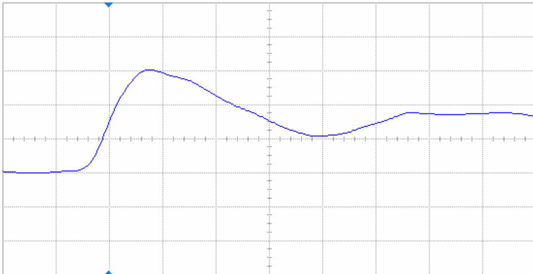
Figure 9(b) DUT 86321 post-annealing rising edge, abscissa scale is 2 V/div and ordinate scale is 2 ns/div.
