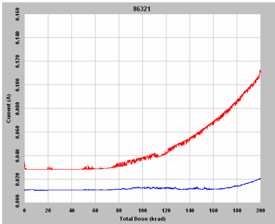
Figure 3 DUT 86321 in-flux I_{CCA} and I_{CCI}
