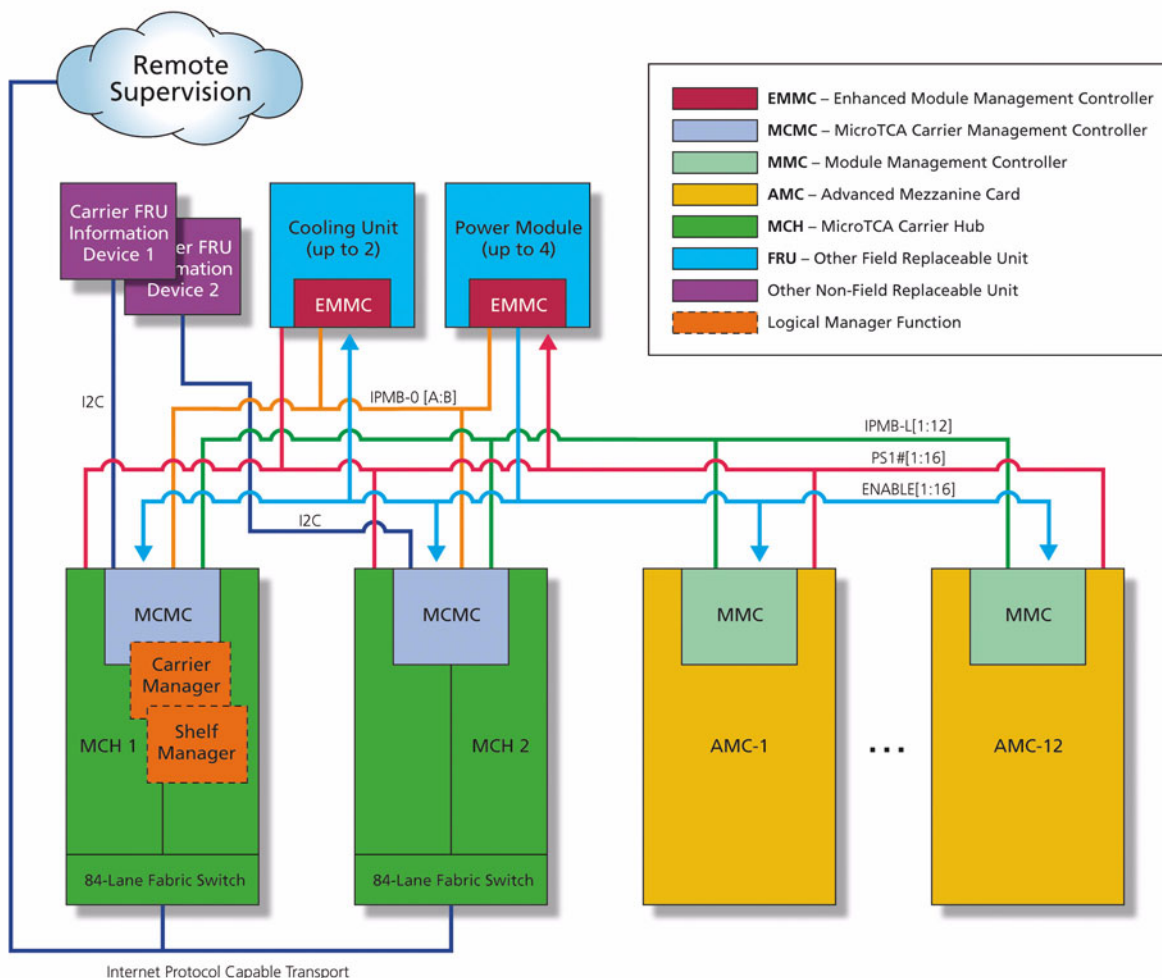
Figure 2 • Management Aspects of an Example MicroTCA Shelf
