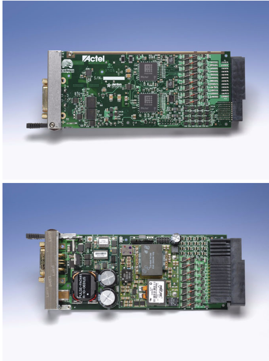
Figure 4 • Actel Power Module Reference Design
