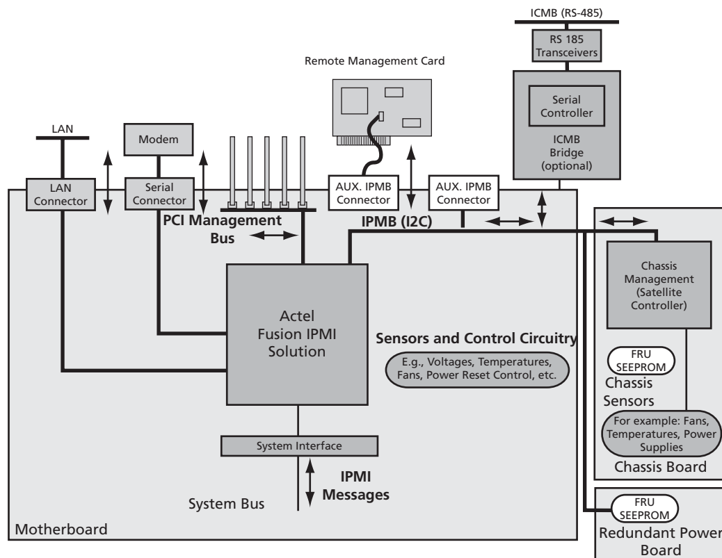
Figure 6 • Fusion-Enabled IPMI Block Diagram
