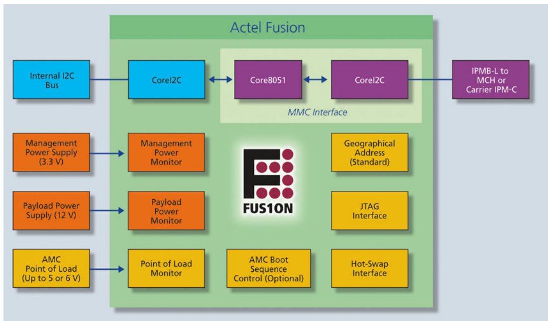
Figure 7 • Fusion-Enabled Advanced Mezzanine Card
