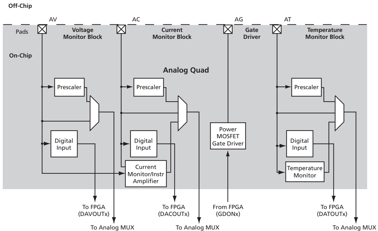
Figure 1: Analog Quad
