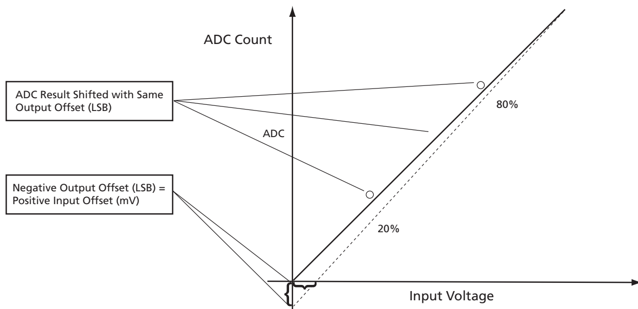
Figure 2: 20% – 80% Calibration Scheme
