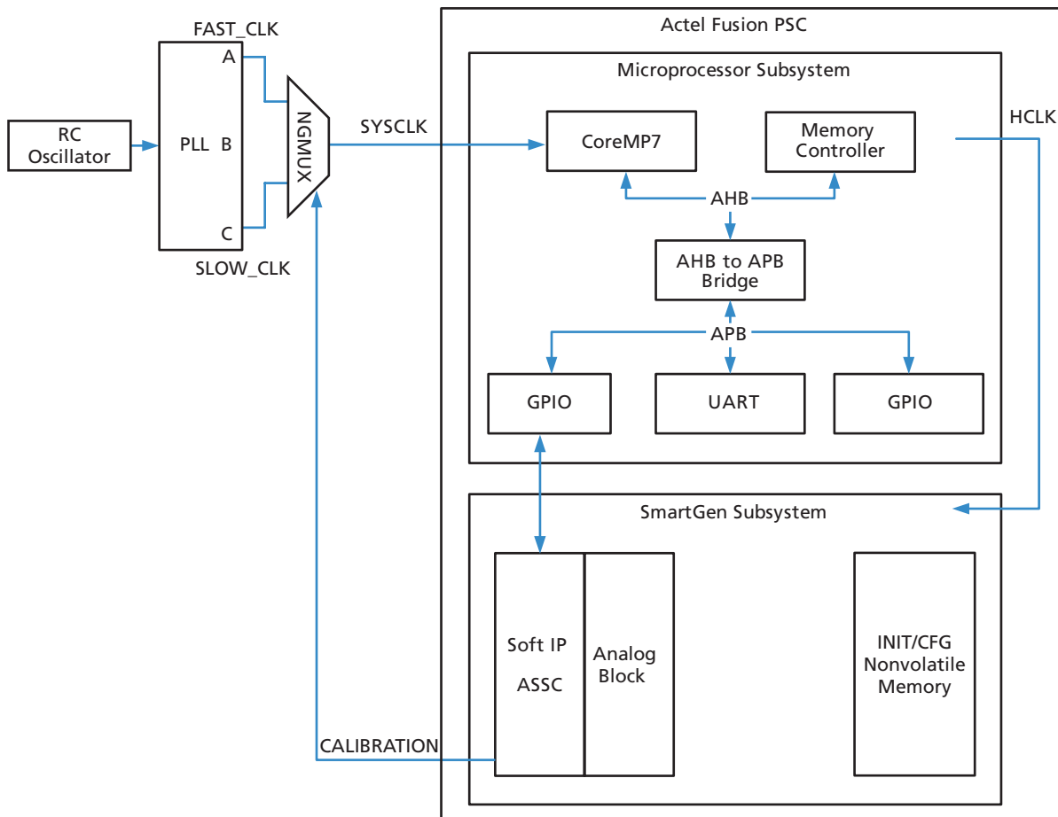
Figure 5 • Partial Microprocessor Control of SmartGen Subsystem
