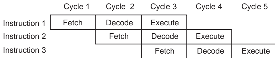
Figure 4: CoreMP7 Pipeline
