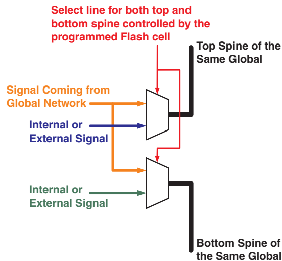
Figure 2 • Spine Selection MUX of a Global Tree
