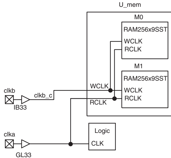
Figure 3 • Simplified Block Diagram of the Example Design
