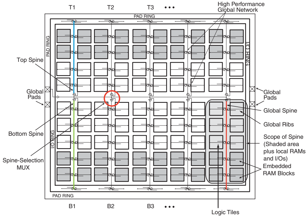
Figure 1 • Spines in a Global Clock Tree Network
