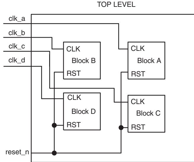
Figure 7 • Block Diagram of the set_net_region Usage Example Design
