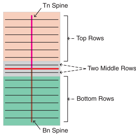
Figure 5 • Illustration of Spines and Middle Die Rows
