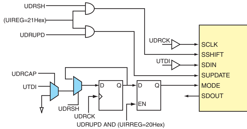
Figure 8 • Sample Implementation of User Interface
