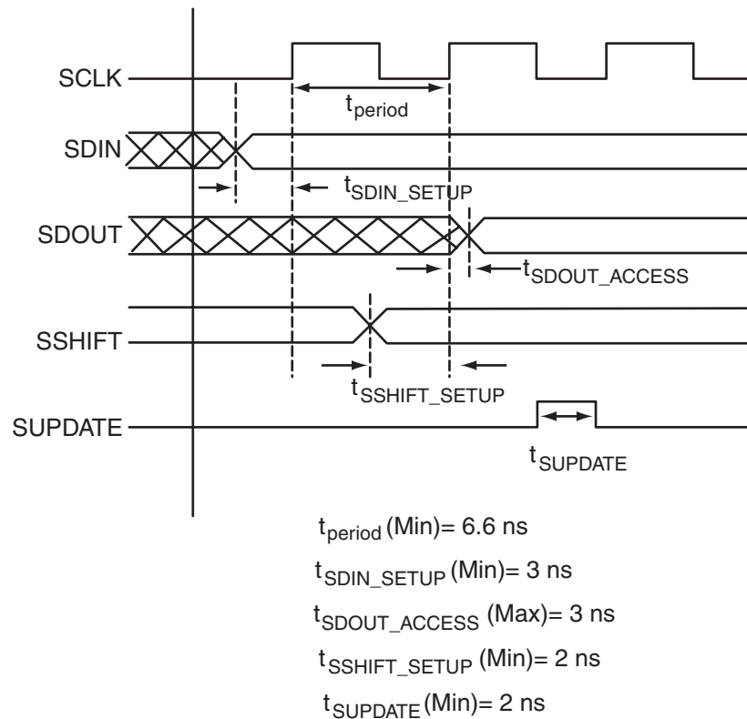
Figure 2 • Timing Diagram
